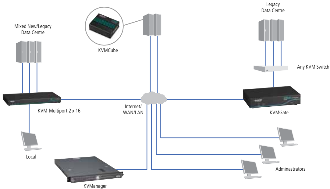
Figure 4 – ServReach KVMoIP manages new, legacy, and mixed data centre infrastructure at the same time.
